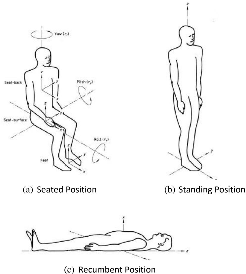
Figure 2 WBV Measurement Directions (Adapted from ANSI S2.72)
